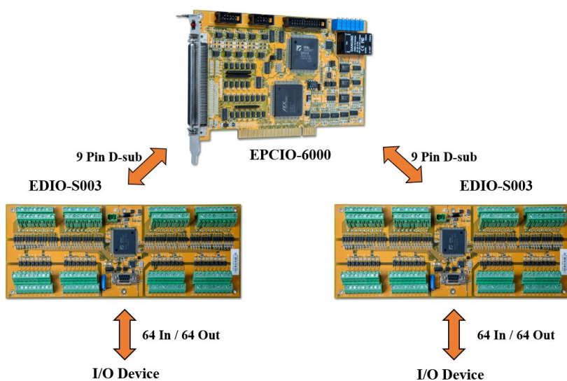
Figure 2.14.1 Remote Master 與 Slave
